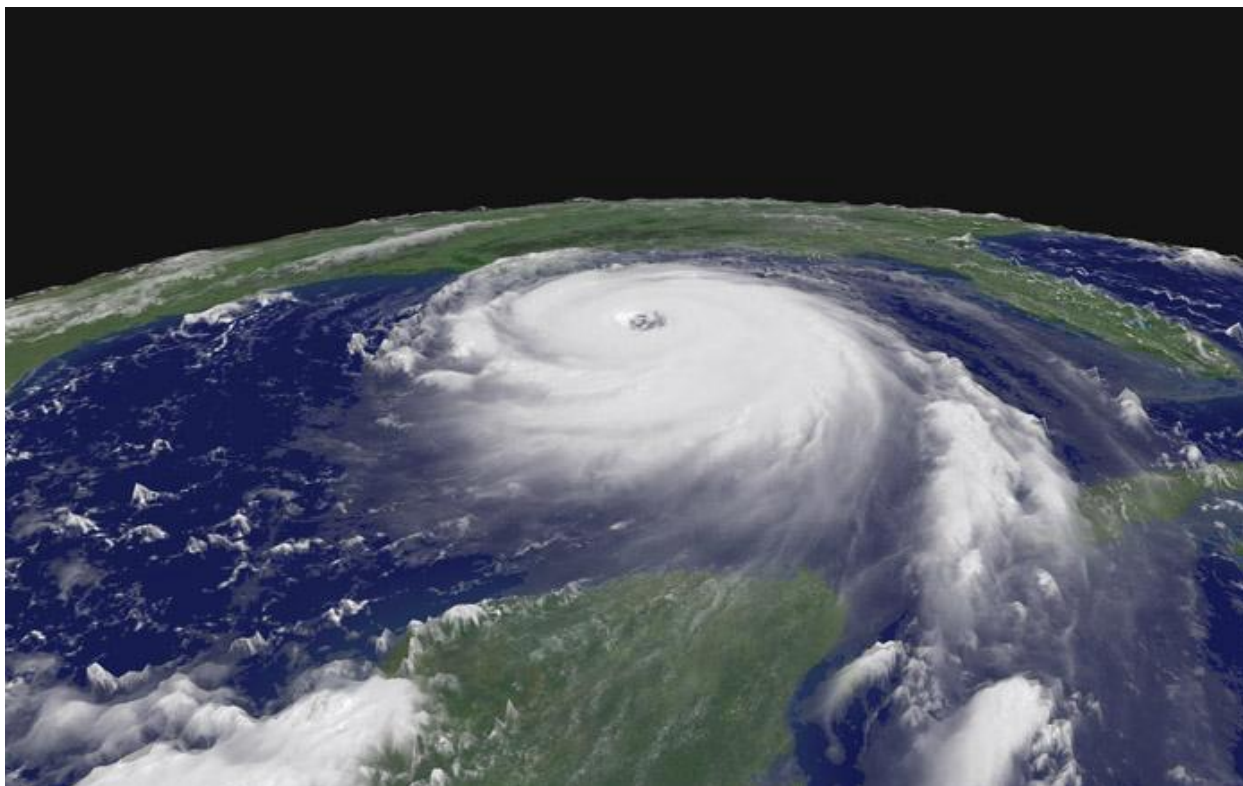
Cyclone Katrina 28/08/2005
