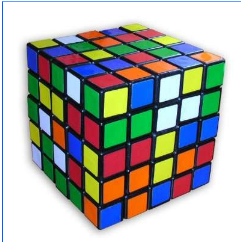
Rubik's cube
