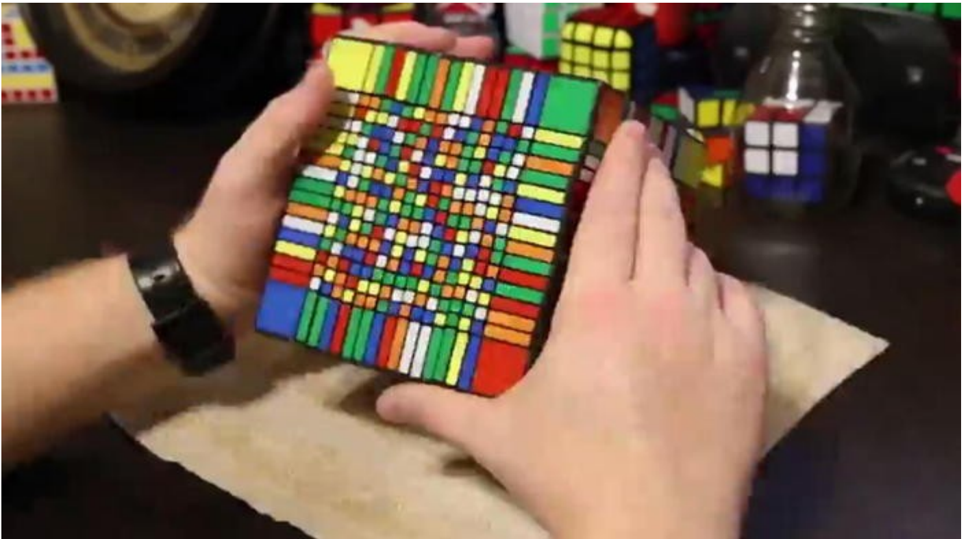
Rubik's cube
