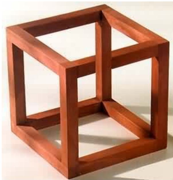
Cube impossible
