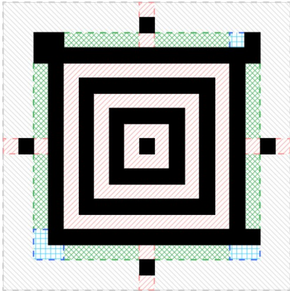
code Aztec
