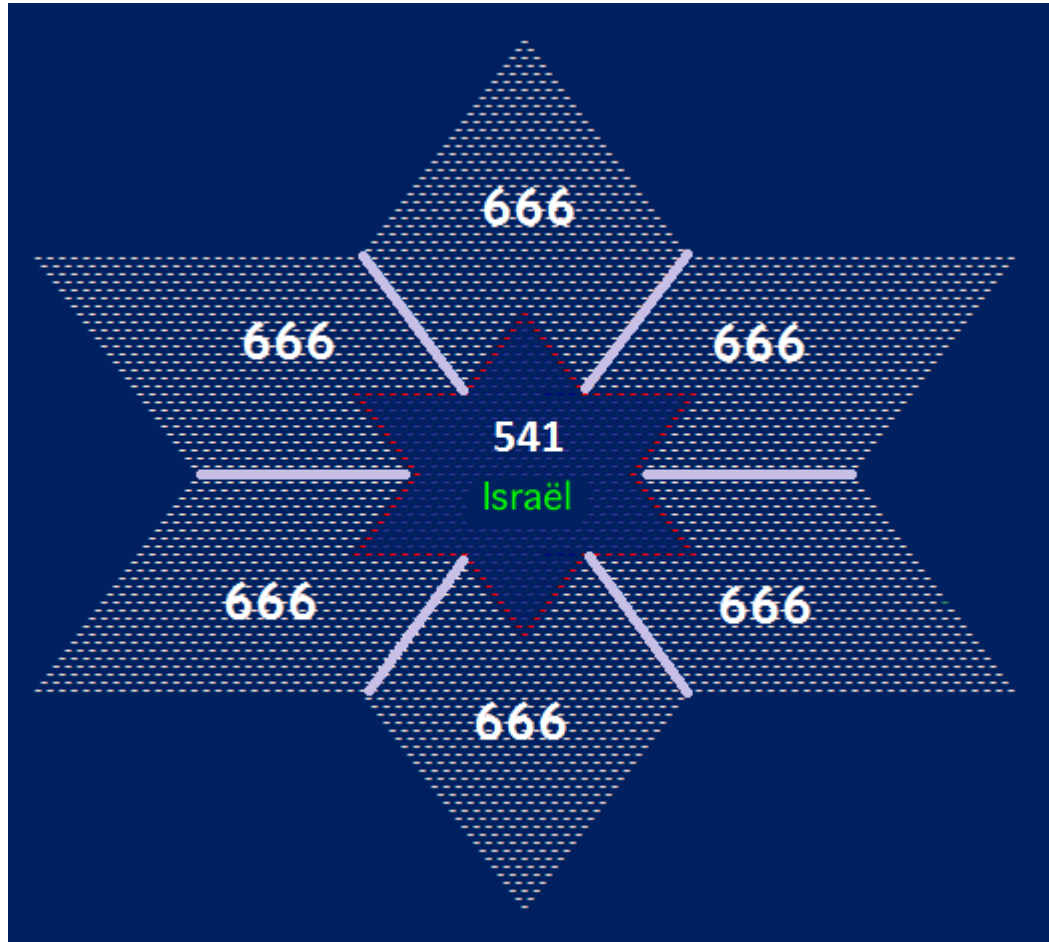
Double hexagone
